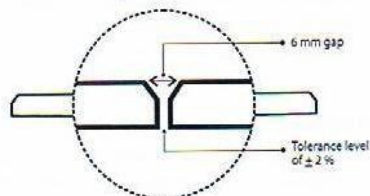
Cross-section of tile after installation
