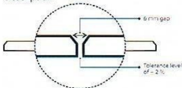
Cross-section of tile after installation
